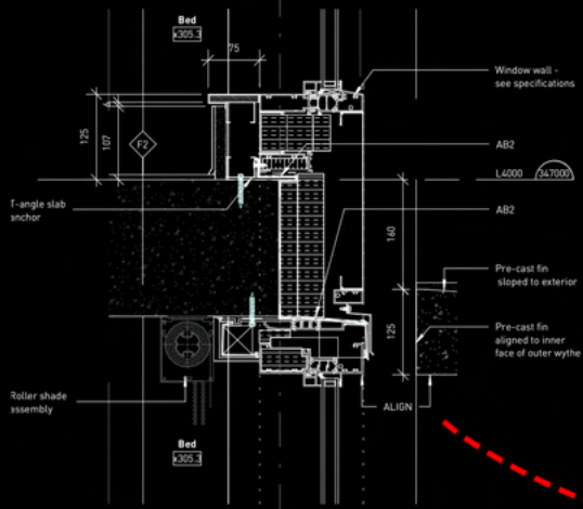
Window wall slab edge detail
