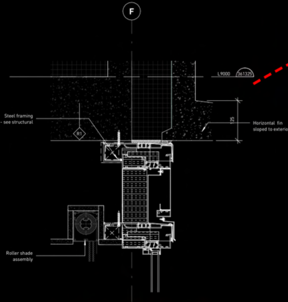
Window wall head detail
