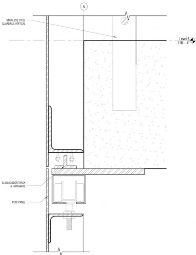
7 Steel Channel @ Operable Panel
