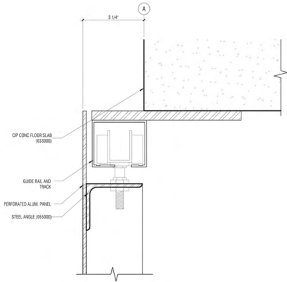
6 Steel Channel Details @ Roof Edge
