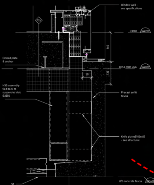
Window wall soffit transition detail
