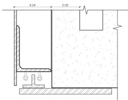
9 Bottom Steel Channel @ Operable Panels
