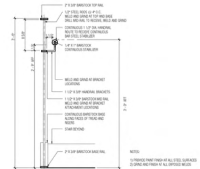
Guardrail and Handrail Detail
